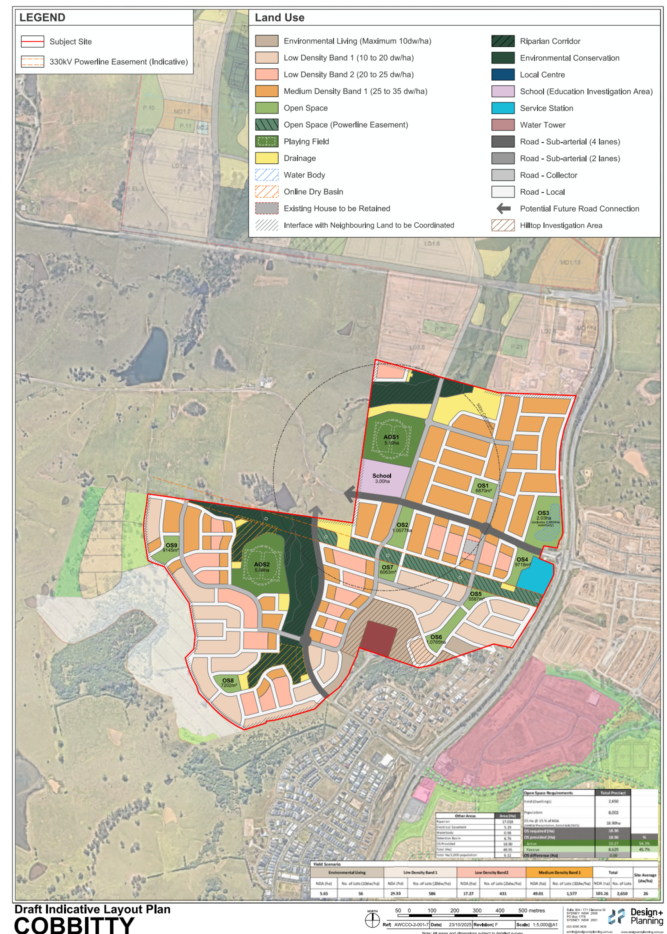
Figure 2.12 Draft Indicative Layout Plan (ILP) Design & Planning)
